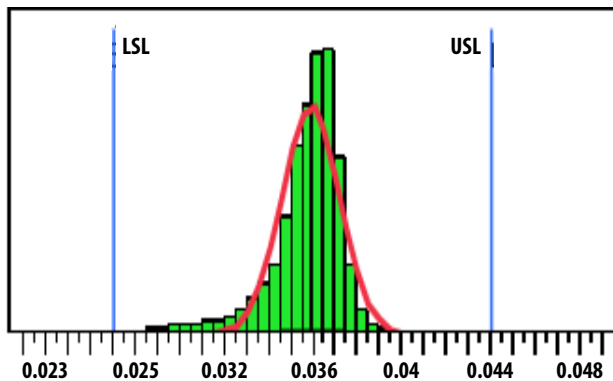
I_d @ V_d = 5\text{ V} , Mean = 36 mA, LSL = 27 mA, USL = 44mA
